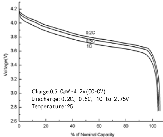
Discharging Characteristic
