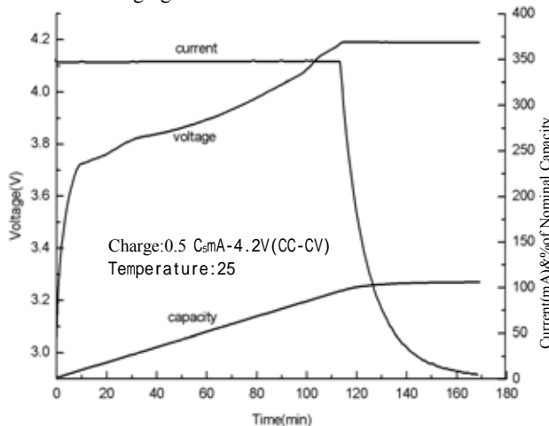
Charging Characteristic
