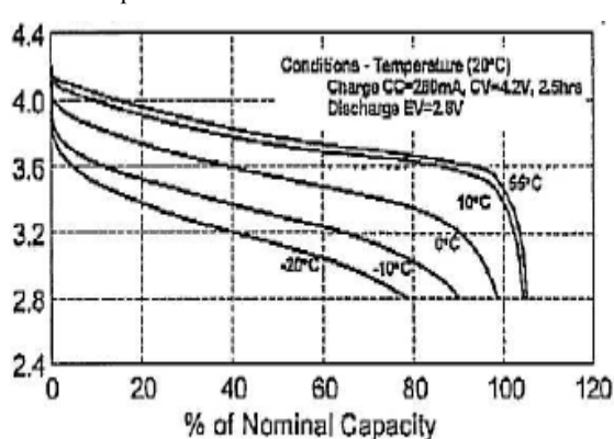
Temperature Characteristic
